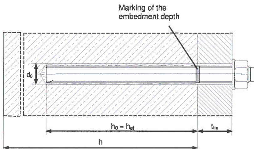
Figure A1: Threaded rod and HIT-V...
